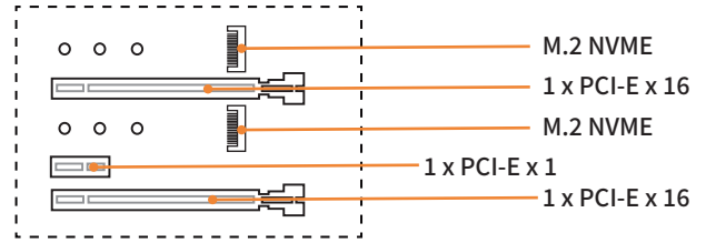
2-4 PCI Expansion Slot
